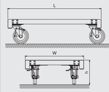
●寸法図 (ALH1275)
